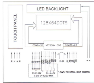
BLOCK DIAGRAM
